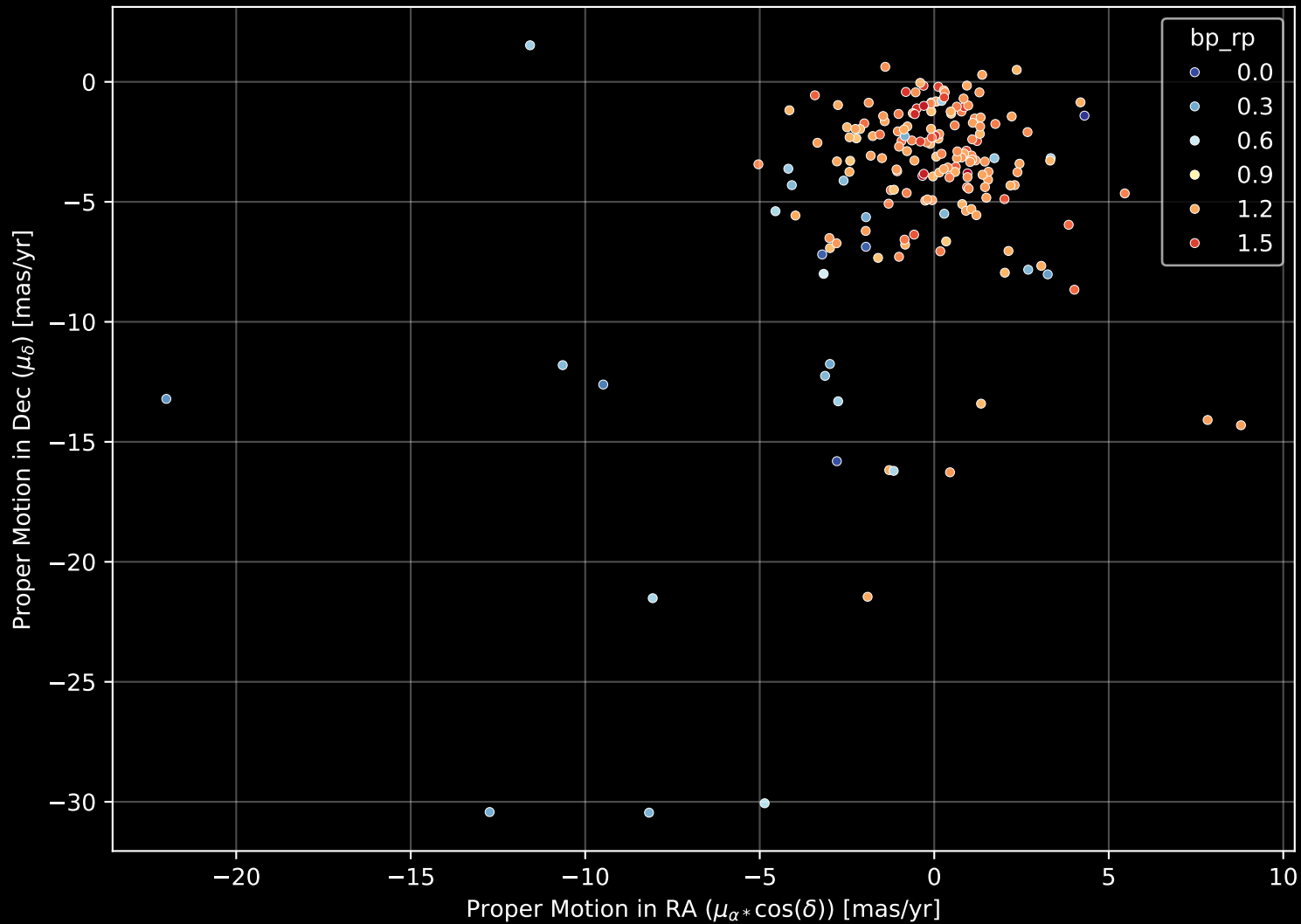
APOGEE DR17 Field: [180+19] Proper Motion Diagram (n= 182)
