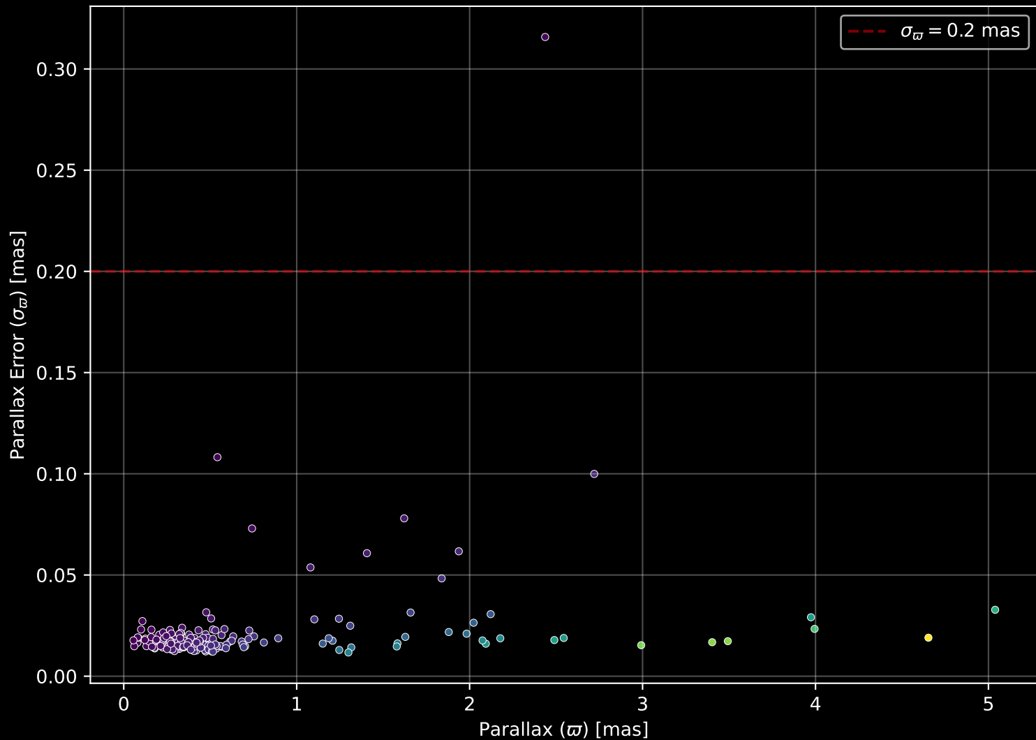
APOGEE DR17 Field: [180+19] Parallax Quality (n= 182)
