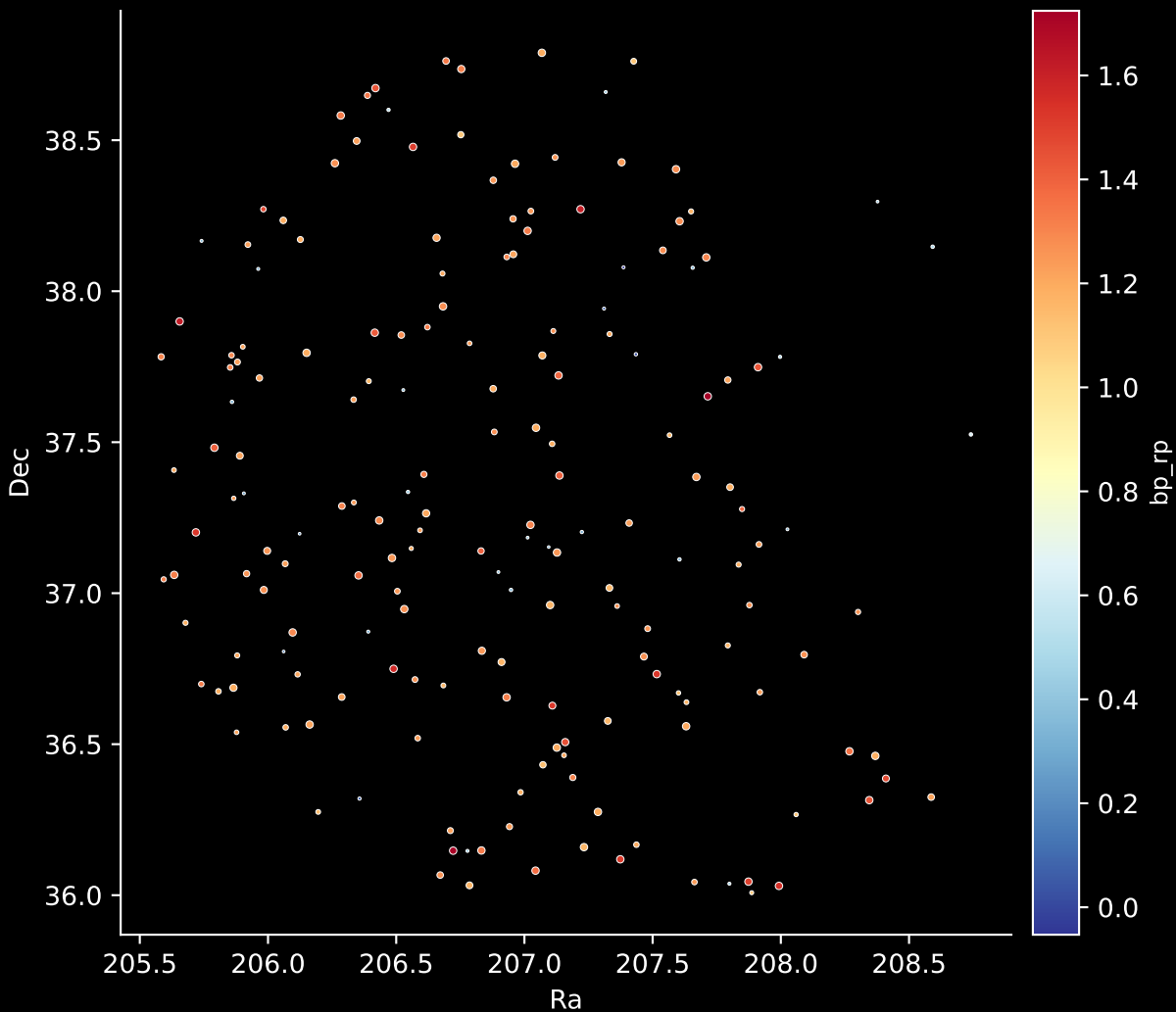
APOGEE DR17 Field: [180+19] Stars: 182
