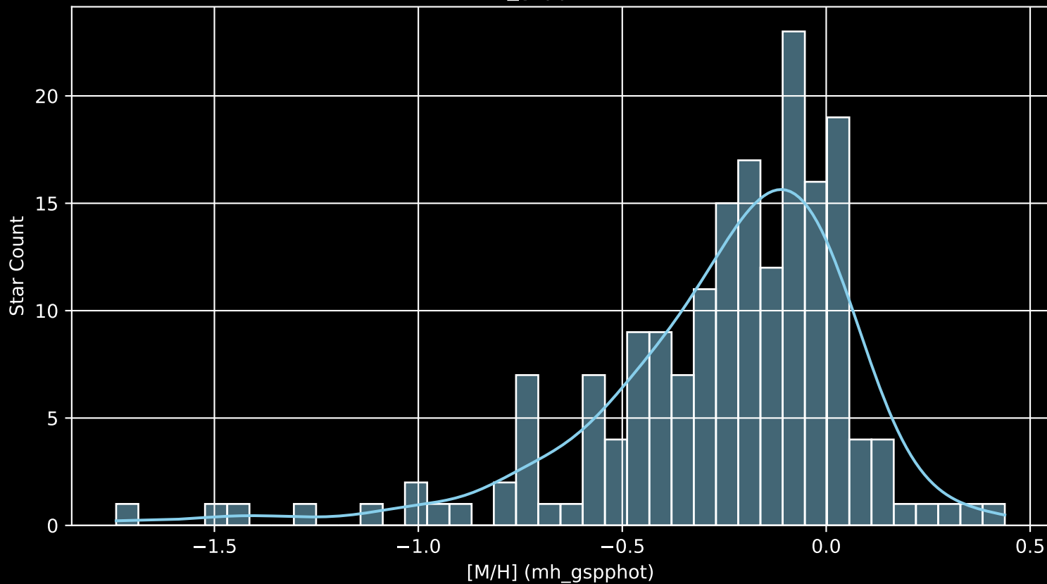
APOGEE DR17 Field: [180+19 [M/H] (mh_gspphot) (n= 182)
