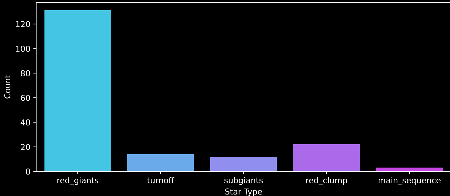
APOGEE DR17 Field: [180+19] Count plot of Star Type
