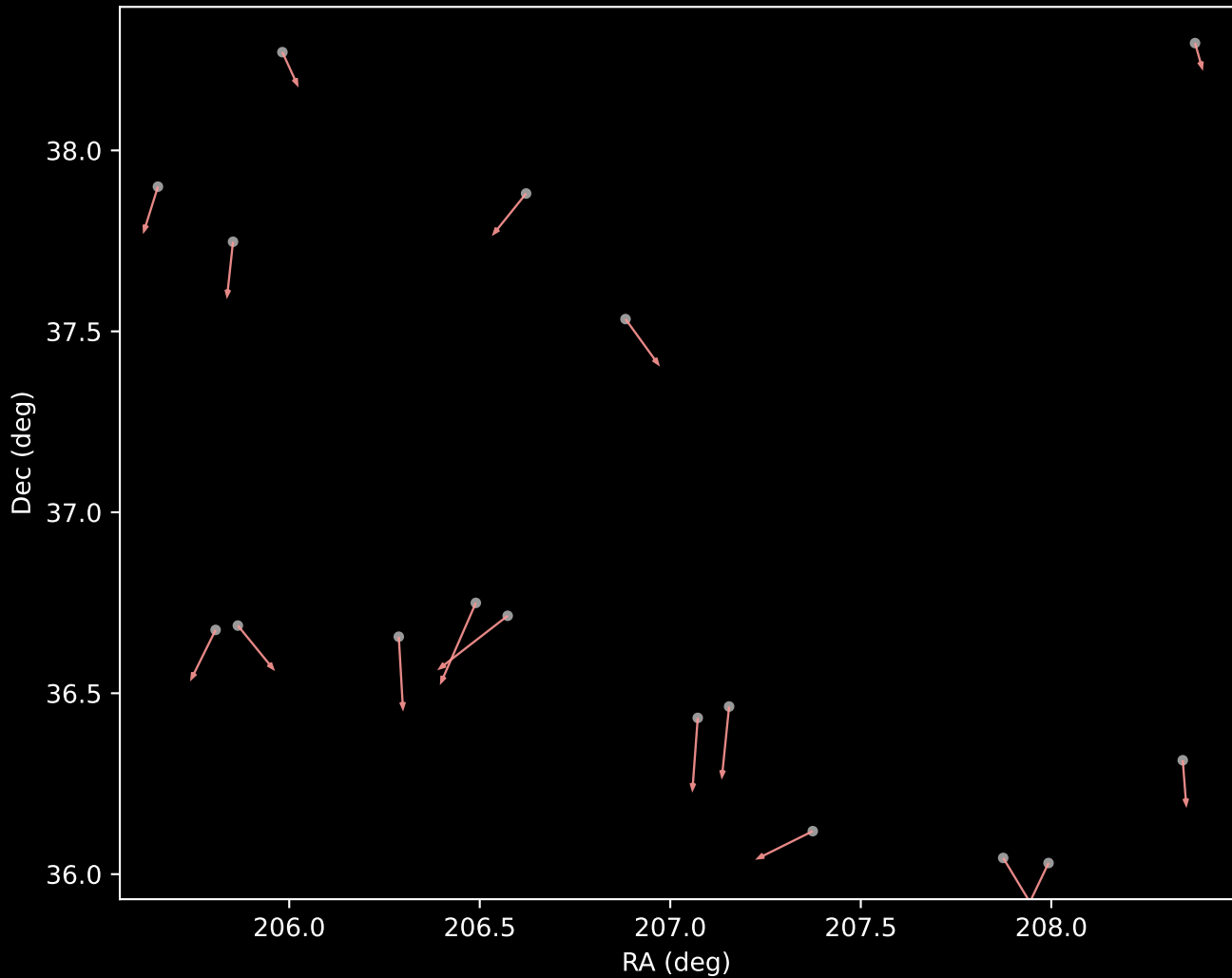
APOGEE DR17 Cluster 7 Proper Motion Vectors (n=17)
