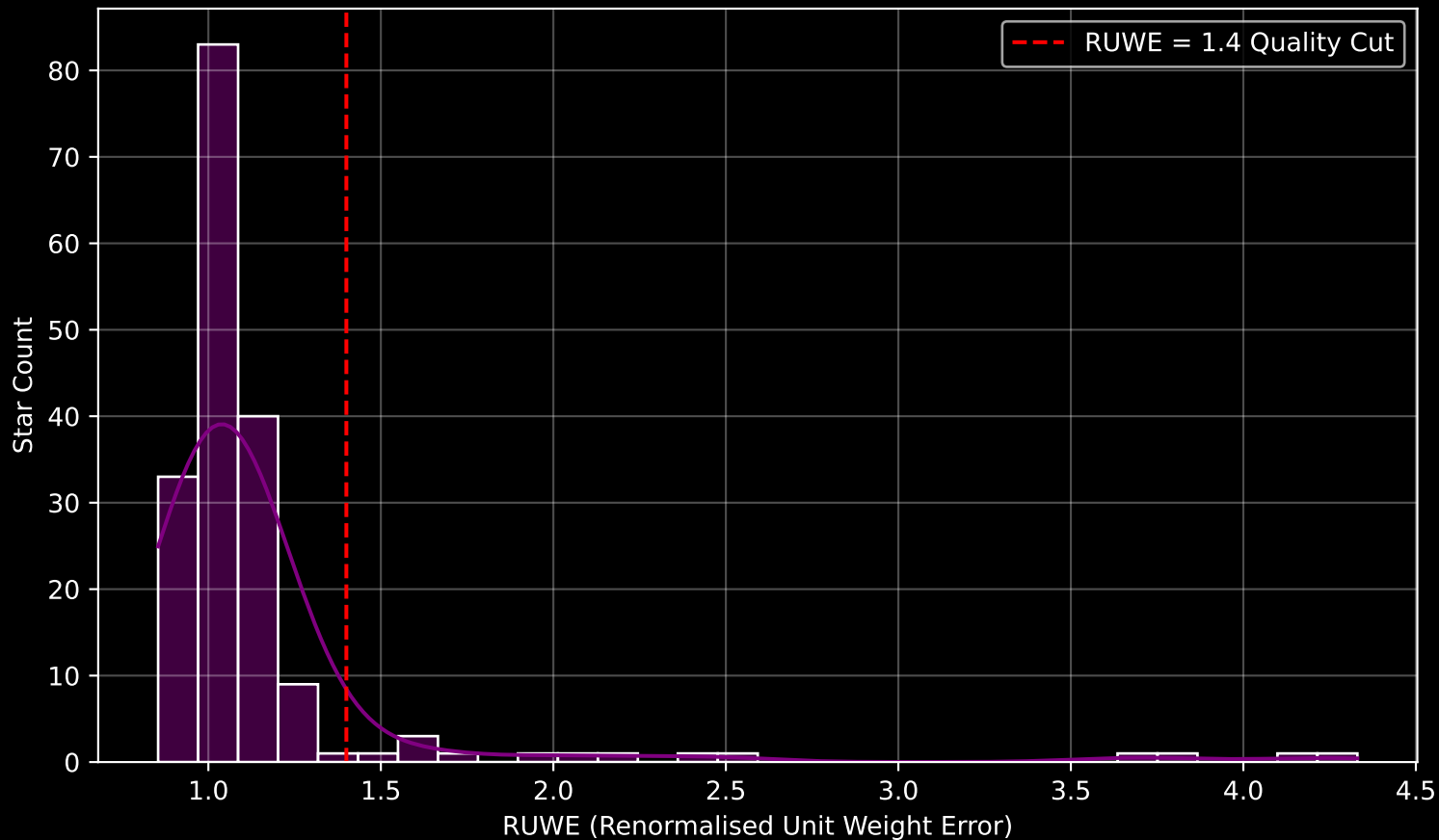
GAPOGEE DR17 Field [180+19] RUWE Distribution (n= 180)
